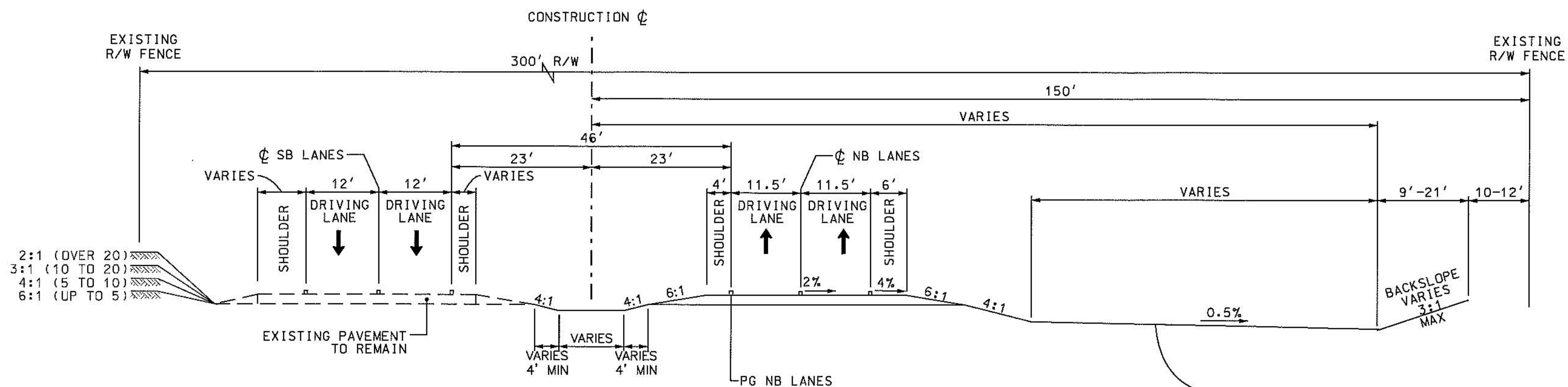
PROPOSED TYPICAL SECTION "A"
