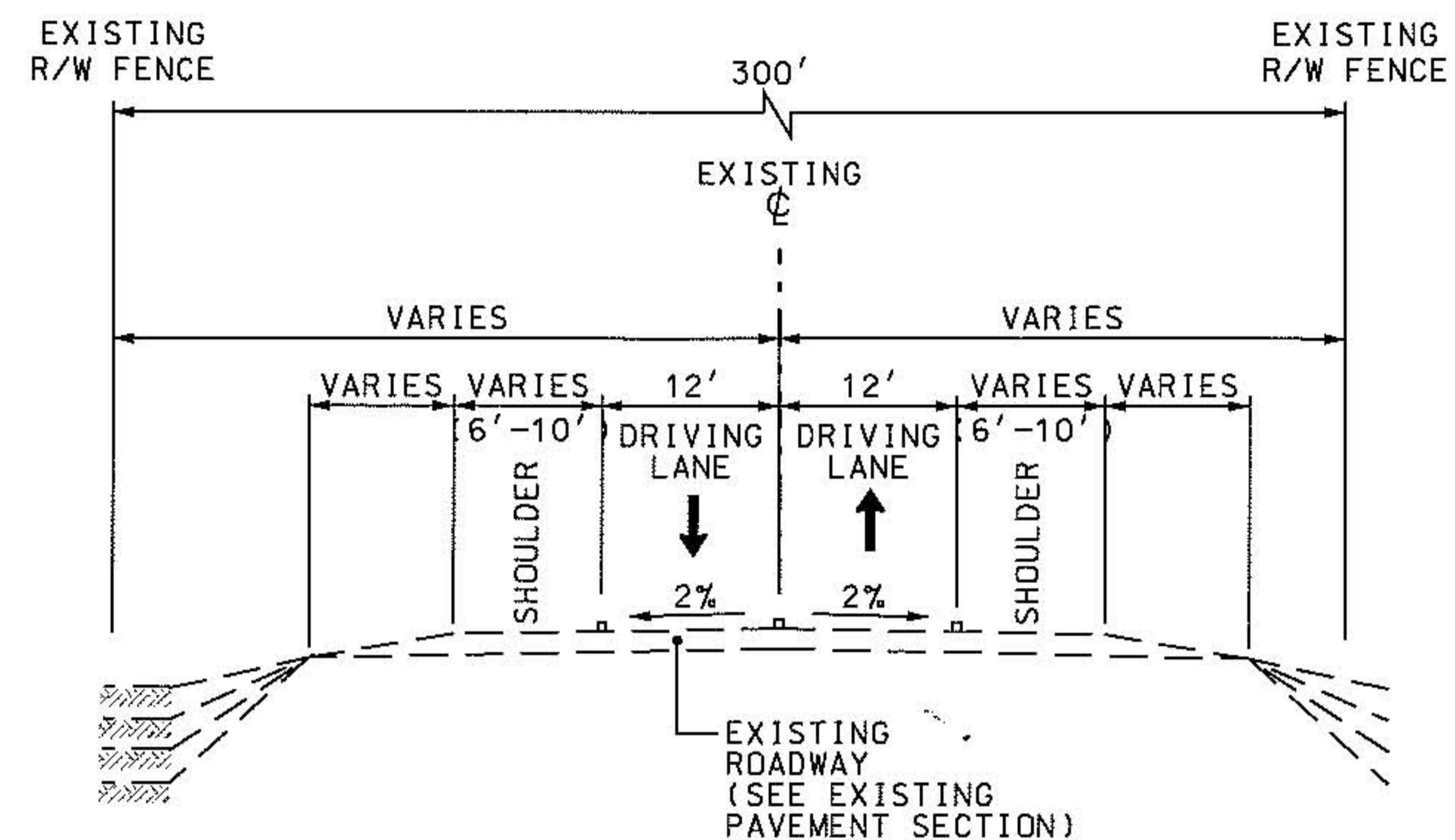
EXISTING TYPICAL SECTION "A"
